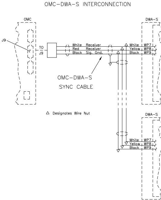
FIGURE 5: OMC – DWA-S INTERCONNECTION
